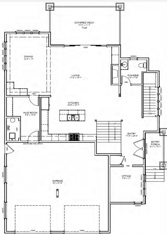
Main Level 1439 SQ. FT.
