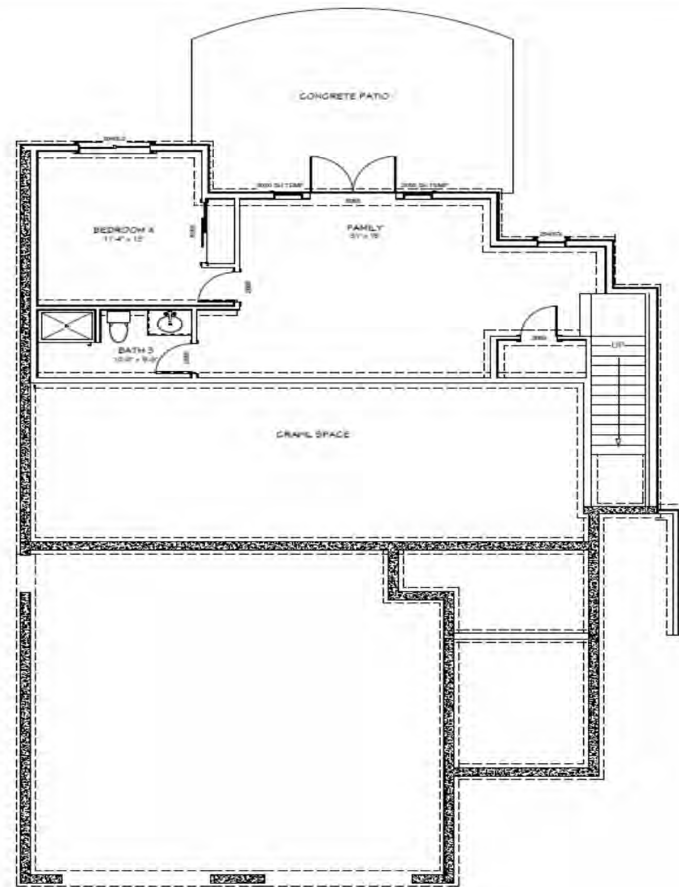
Lower Level 719 SQ. FT.
